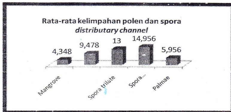
Gambar 2. Rata-rata kelimpahan polen dan spora distributary channel
