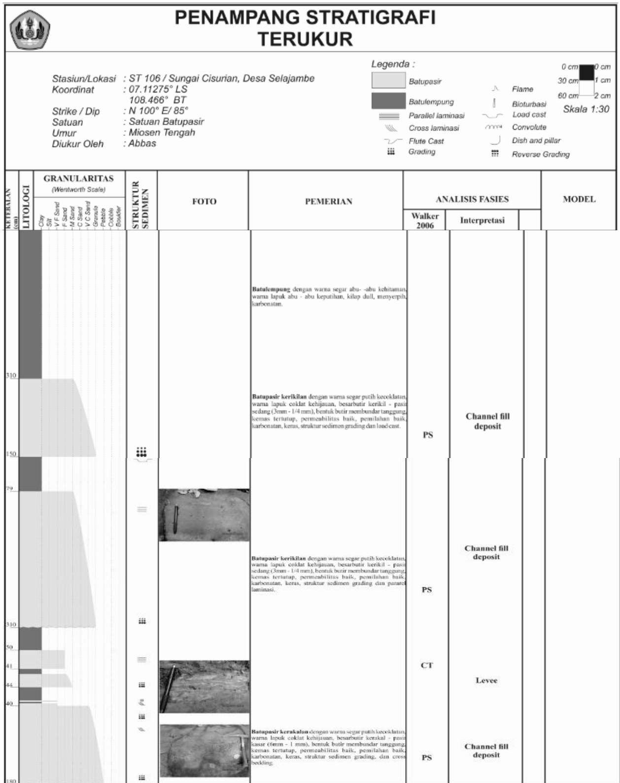
Gambar 6 (c). Penampang Stratigrafi Terukur Satuan batupasir.
