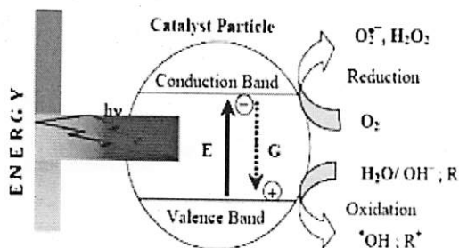
Figure 1. Simplified Mechanism for the Photocatalysis of a Semiconductor Catalyst [4]
